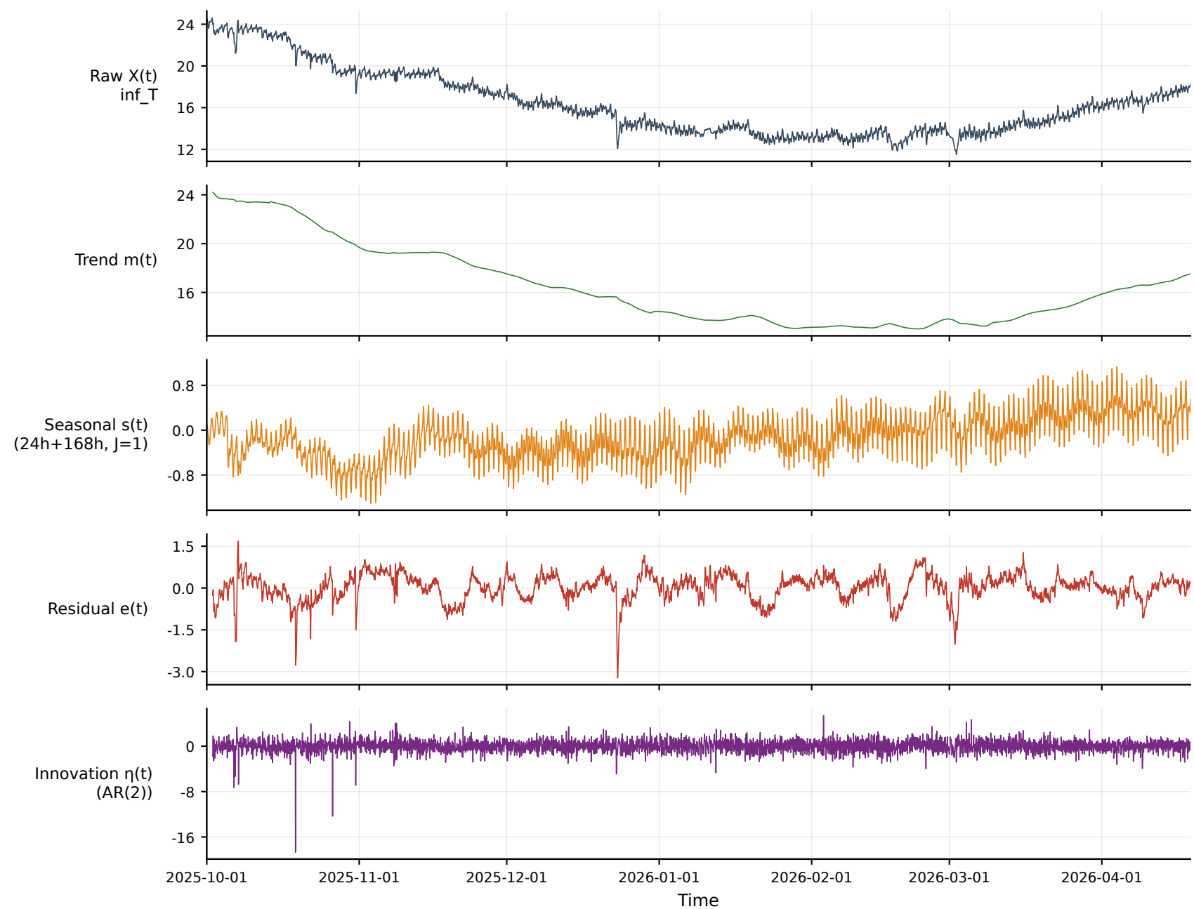
Multi-scale decomposition — inf_T (influent, hour) [2025-10-01~2026-04-19]
